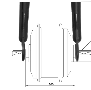
Example showing template placed in fork which clears motor
